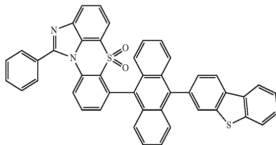
[Chemical Formula 1-6-14]
