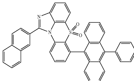
[Chemical Formula 1-6-2]
