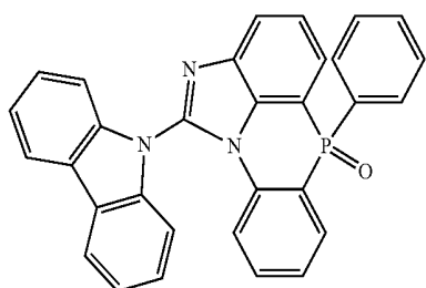
[Chemical Formula 2-5-51]
