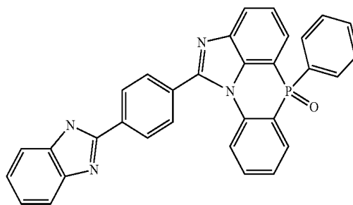
[Chemical Formula 2-5-47]
