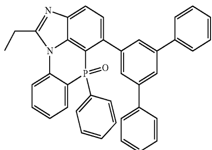
[Chemical Formula 2-9-5]
