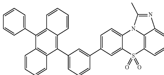
[Chemical Formula 1-2-18]
