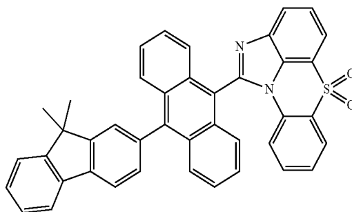
[Chemical Formula 1-5-5]
