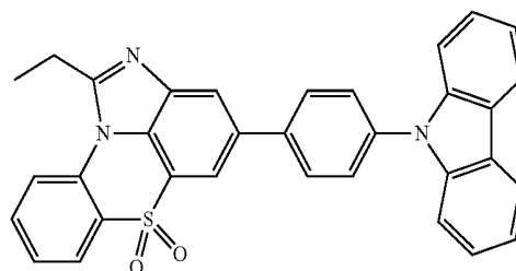
[Chemical Formula 1-10-7]
